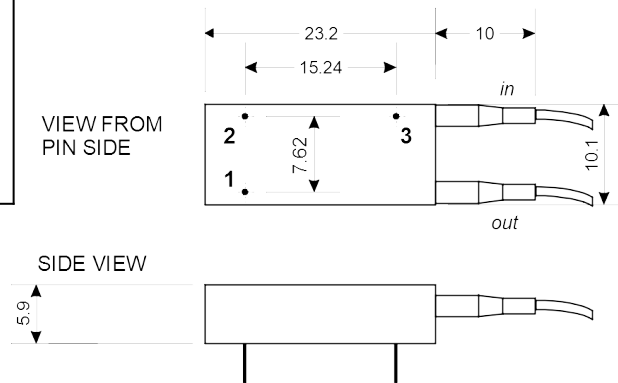
Figure 7: VXP-1: mechanical outline
