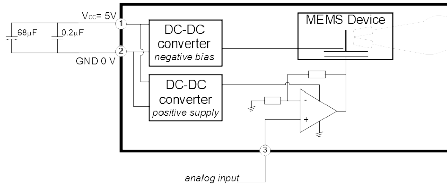
Figure 9: Schematic Electrical Diagram
