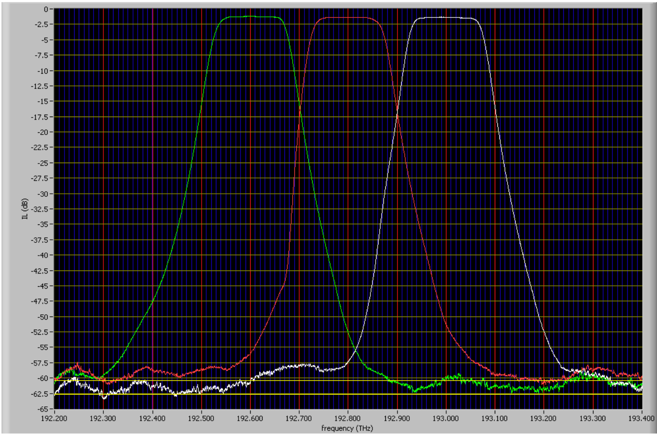
PM Mux/Demux 200GHz spacing based on TFF
