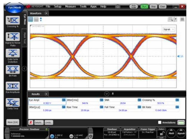
Data Rate = 14 Gb/s, V_{in} = 220\text{ mV}_{pp}
