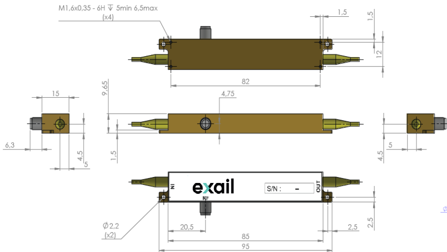
Housing #A: Standard Modulator housing
