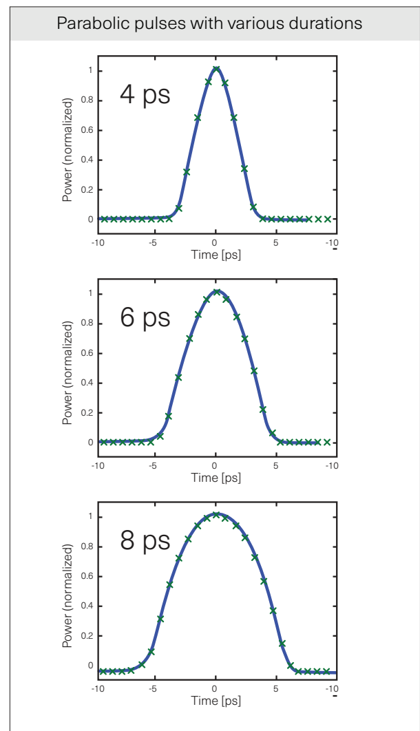
Examples of some of the pulse shapes which can be generated using a WaveShaper 1000A/SP in combination with a short pulse laser and appropriate compressive elements.
